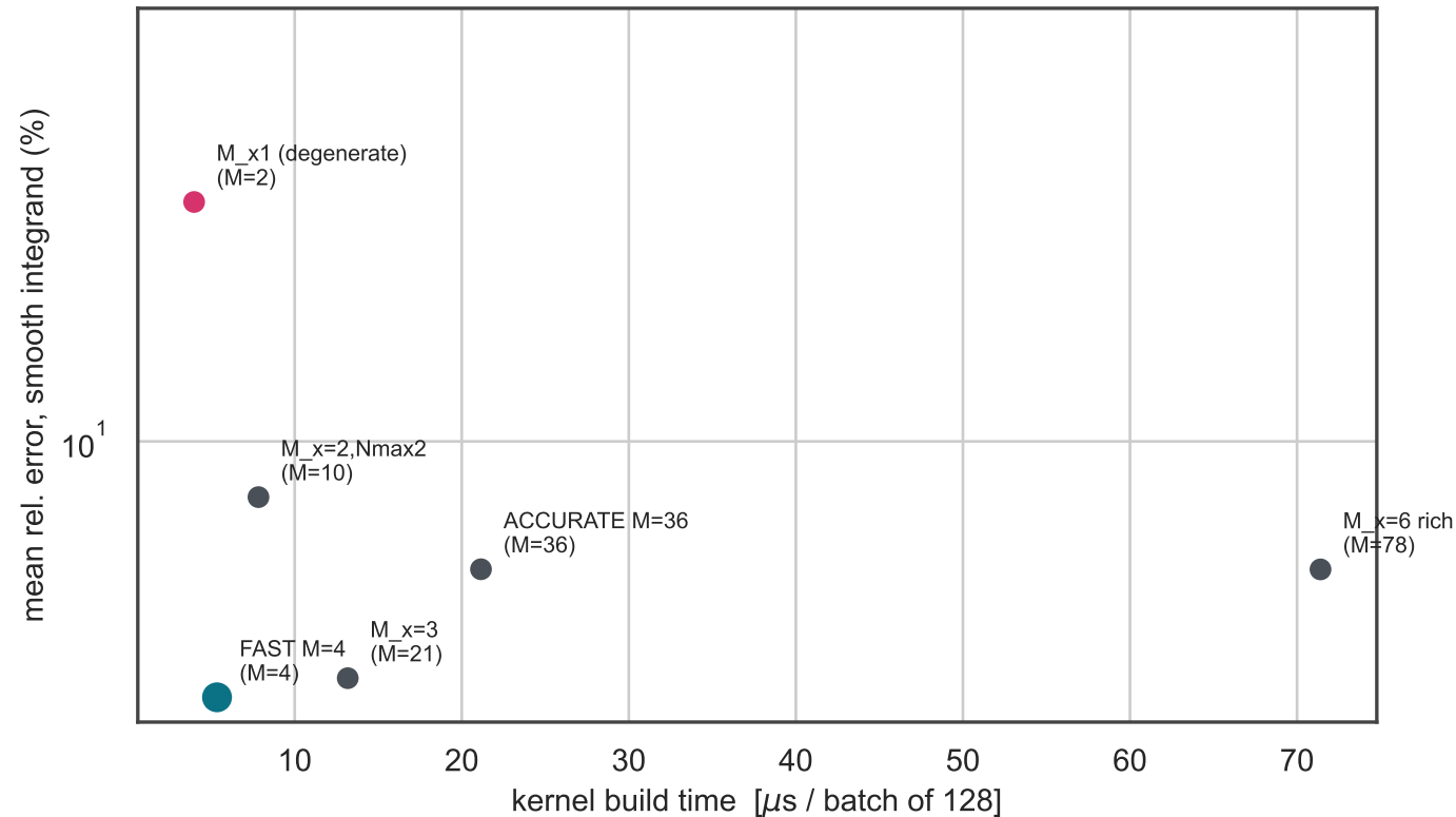
F5 · Cost / accuracy frontier — FAST M = 4 at the knee
